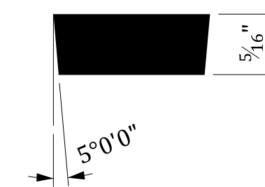
SECTION X-X
