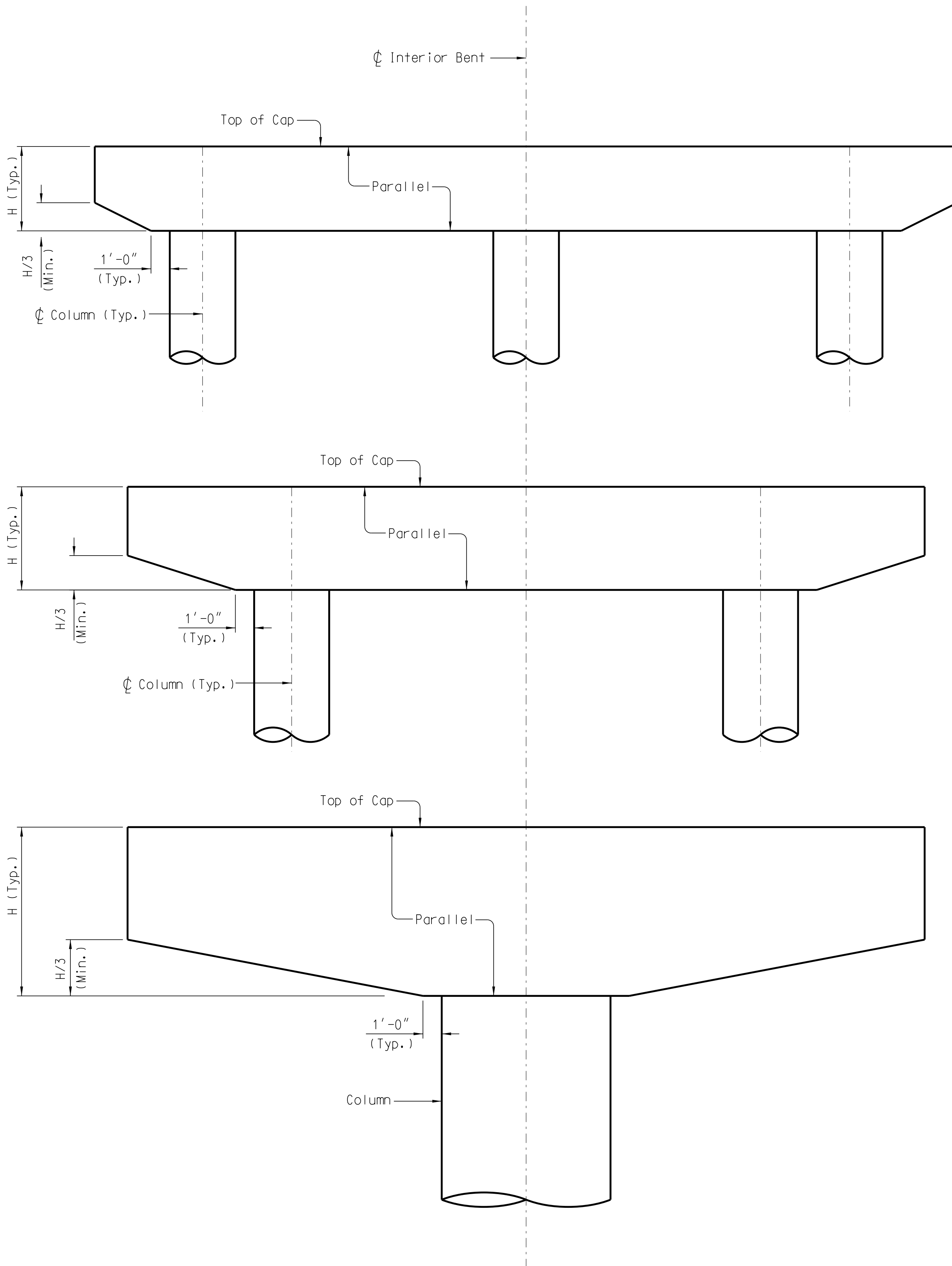
INTERIOR BENT CAP OVERHANG DETAILS
