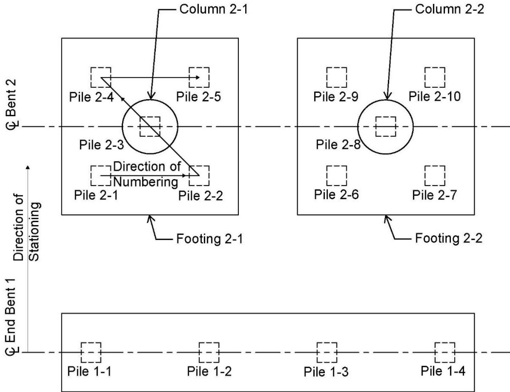
Figure A5.3-4. Standard Pile Labeling Convention
