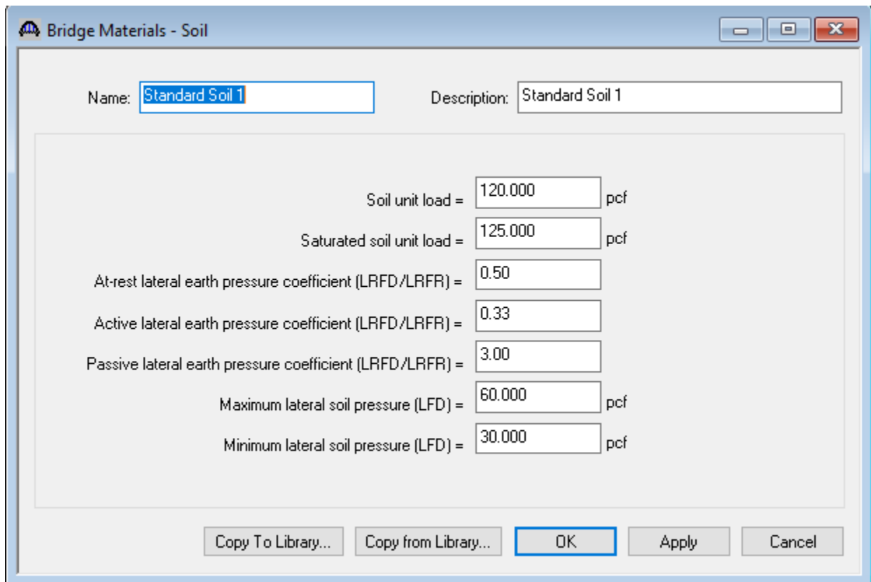
Figure 17.2.1.1-1. Concrete Box Culvert Soil Properties for BrR
