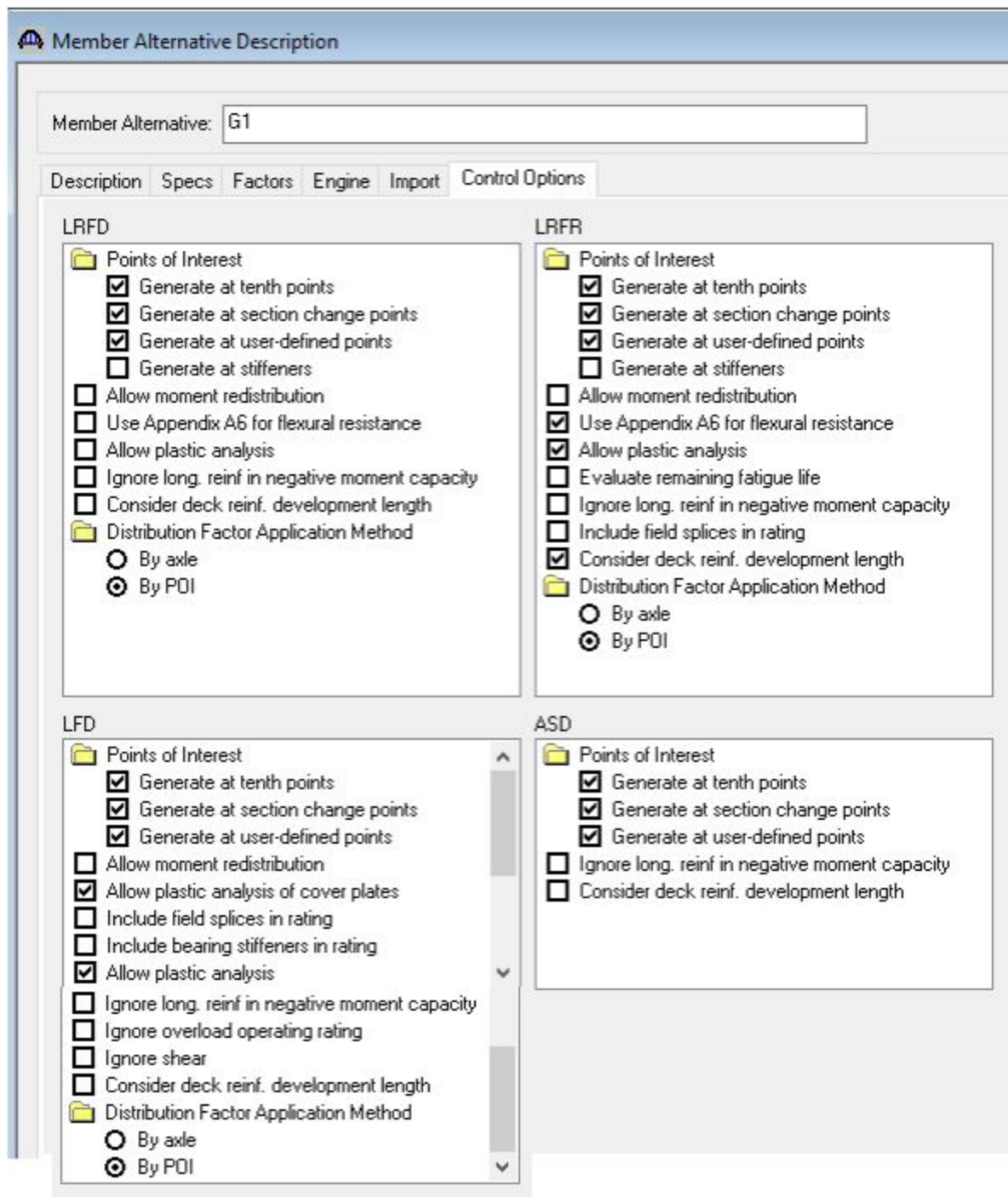
Figure 11.2.2.2-1. Control Options in BrR for Steel Girder Superstructure
