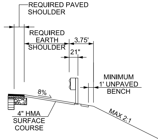
STANDARD GUARDRAIL DETAIL WITH ASPHALT NON-MOW STRIP
