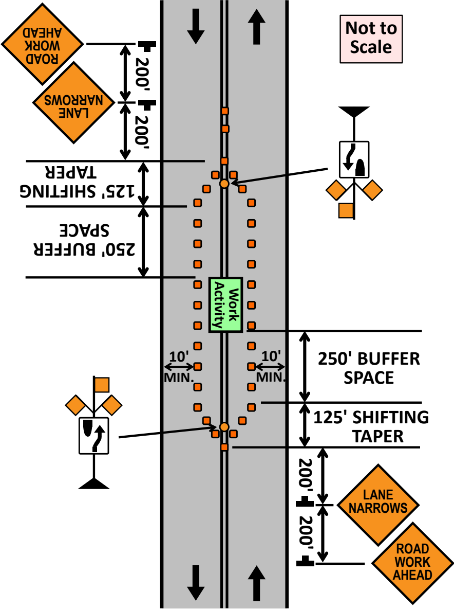
Drawing 8. Work in Center of a Minor Urban Street, 35 MPH or Less, Maintaining Two-Way Traffic
