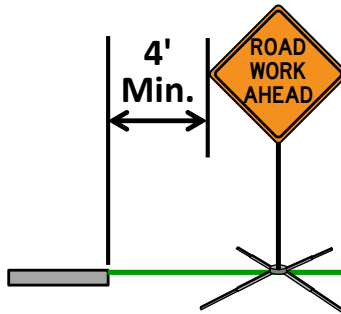
Earth Shoulder
