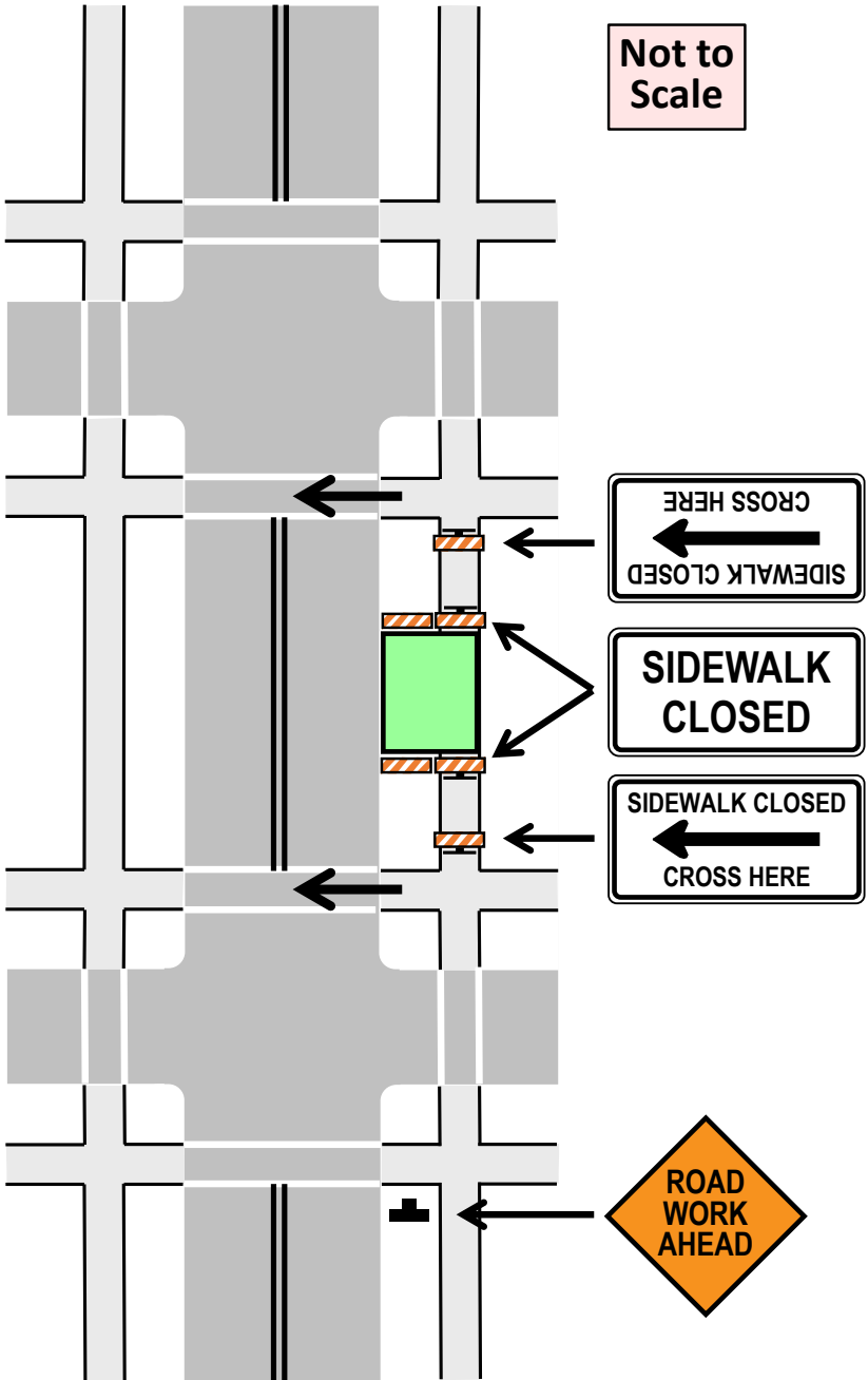
Drawing 25. Sidewalk Closure, Pedestrian Detour
