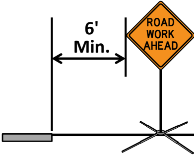
Paved Shoulder
