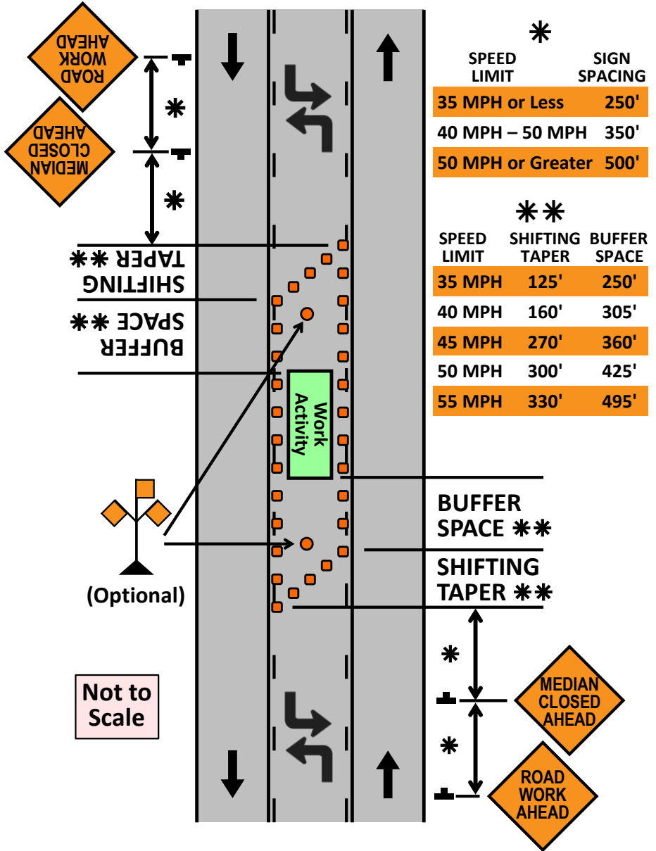
Drawing 10. Center Turn Lane Closed on a Three-Lane, Two-Way Road
