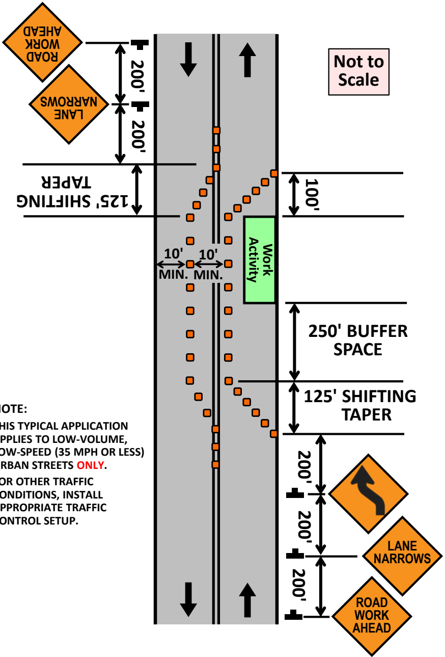
Drawing 9. Work in Travel Lane on a Minor Urban Street, 35 MPH or Less, Maintaining Two-Way Traffic
