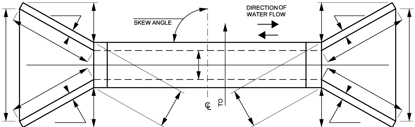
TOP VIEW SHOW DIMENSIONS
