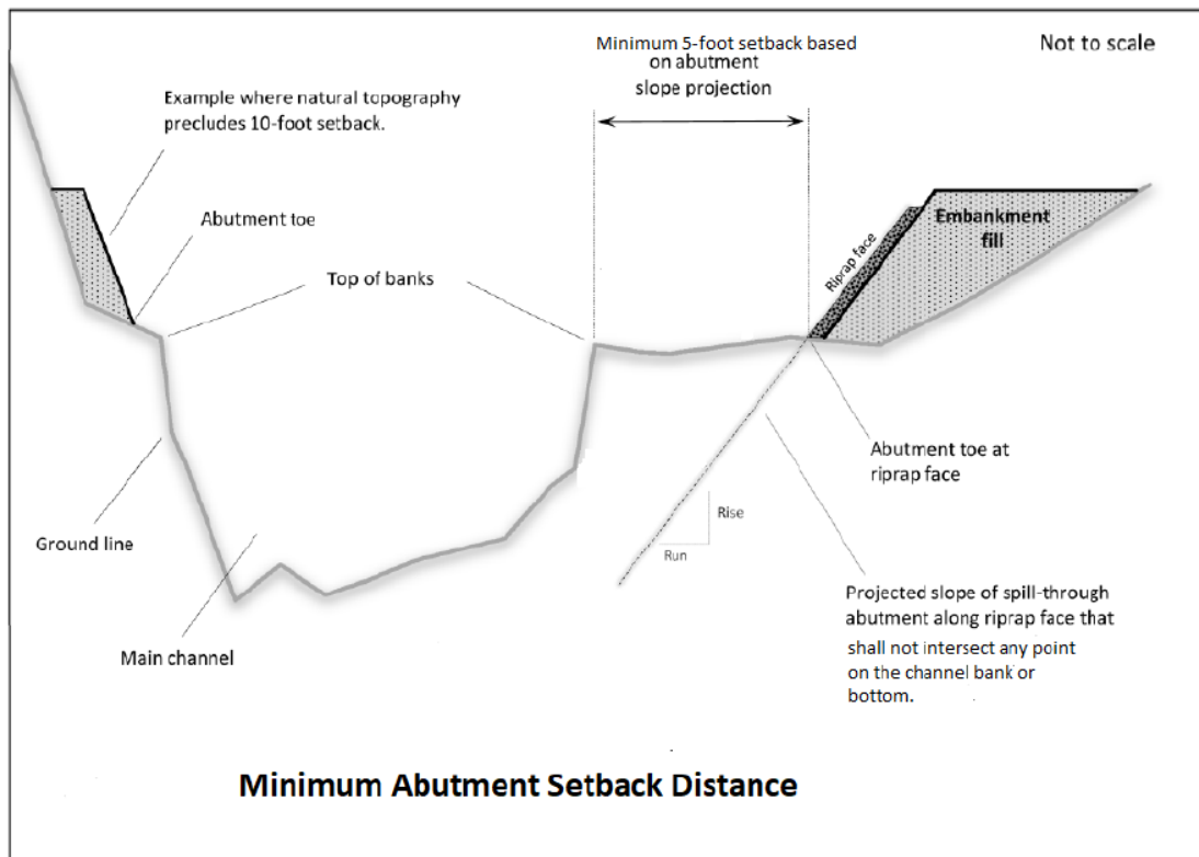
figure 1. Illustration showing minimum abutment setback distances in reference to (1) the channel bank and (2) the projection of the spill-through abutment slope
