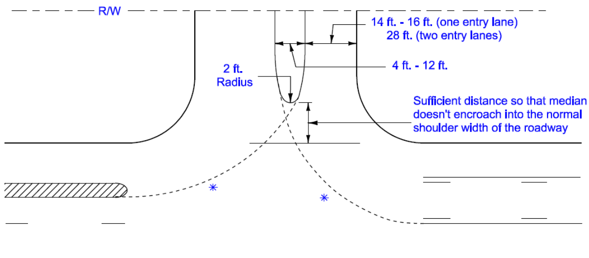
Figure 3-6: Driveway Median Design
